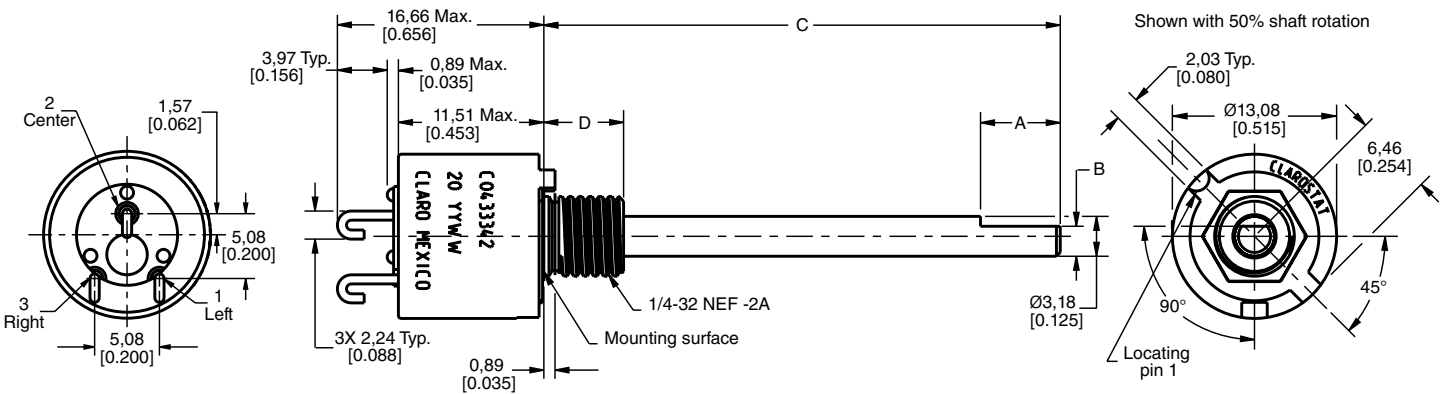
Dimensional Drawings (For reference only: mm [in].)
