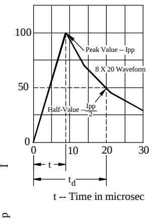
FIGURE 2 Pulse Wave Form
