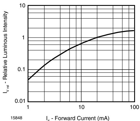
Fig. 4 - Relative Luminous Flux vs. Forward Current
