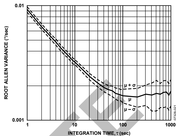
Figure 10. Root Allen Variance, VCC = 5 V, 25°C
