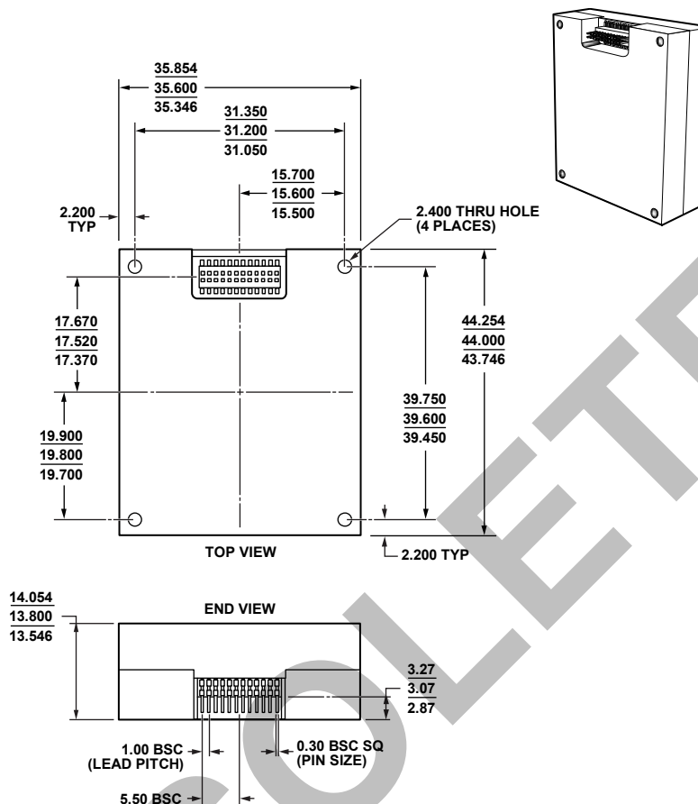
Figure 18. PCB Module with Connector Interface (ML-24-3)
