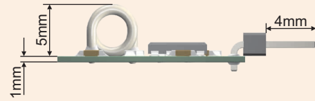
RX-3aAu (standard, unshielded coil, angular pins )
