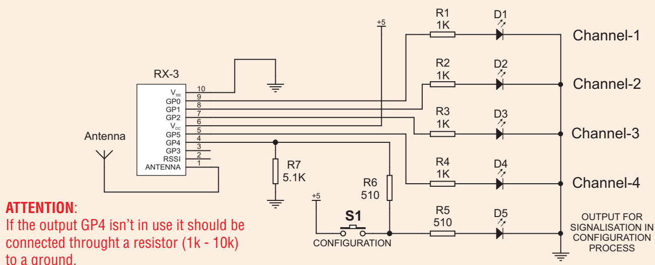
Figure 1. Basic start-up application of the RX-3.
