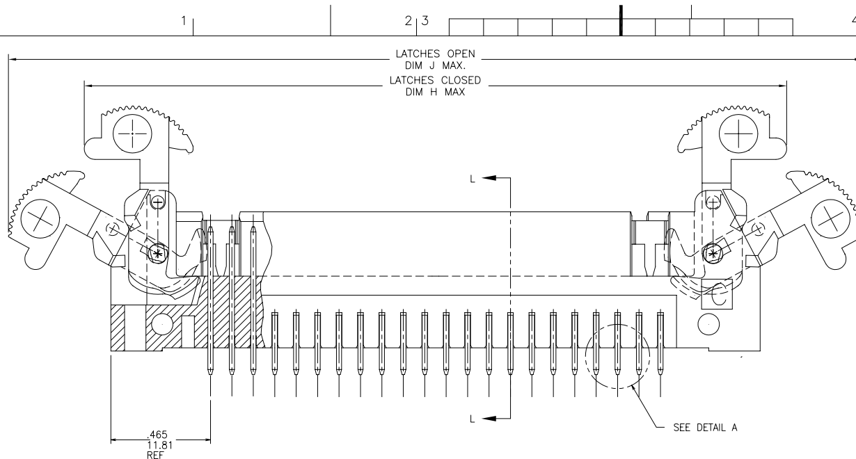
VIEW Y-Y
