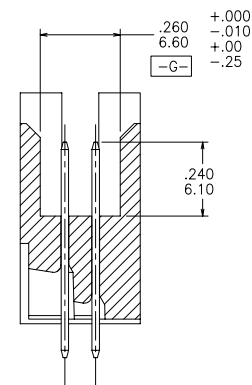
SECTION L-L
