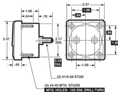
2 - 1/2" Model 1287
