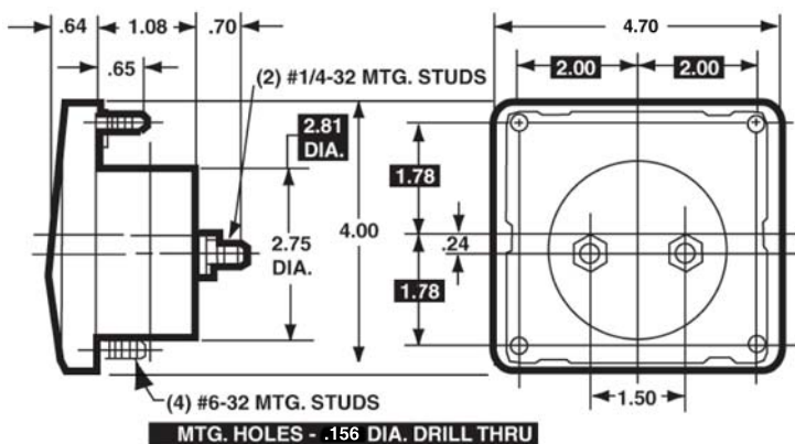
4 - 1/2" Model 1389
