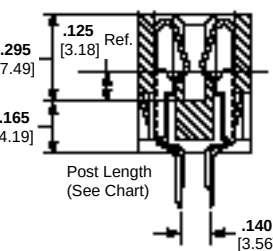
Flow Solder Post .140 [3.56] Row-to-Row Spacing
