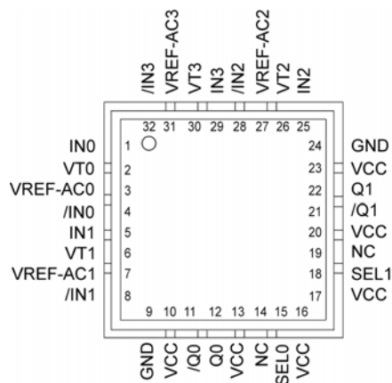
32-Pin QFN
