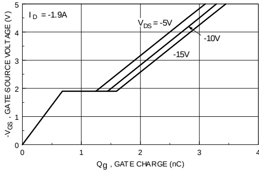
Figure 7. Gate-Charge Characteristics.
