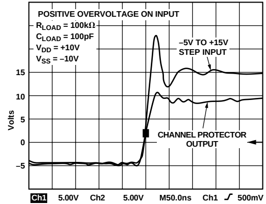
Figure 3. Positive Overvoltage Transience Response
