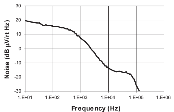
Noise Spectrum
