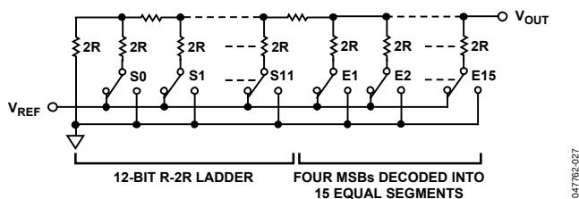
Figure 6. Dac Ladder Structure
