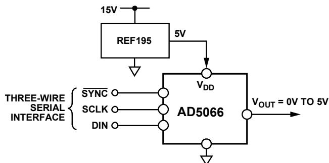
Figure 14. REF195 as Power Supply to the AD5025/45/65
