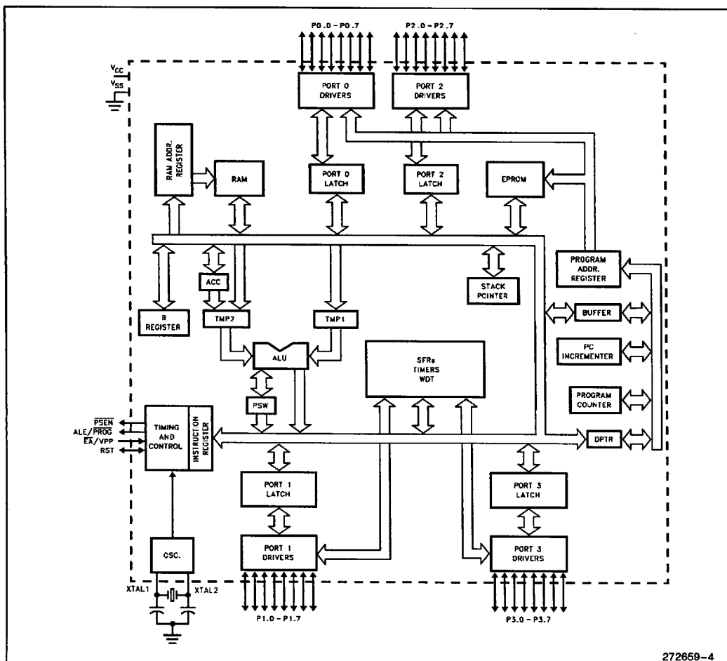
Figure 1. 8XC51RX Block Diagram
