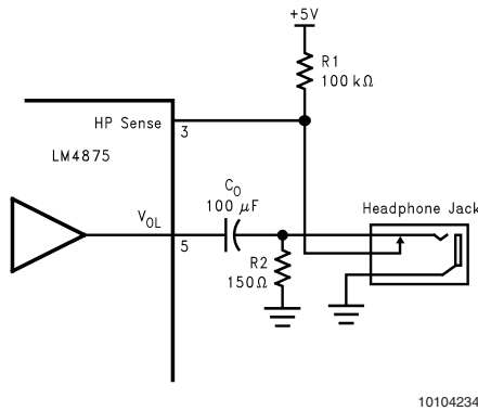
FIGURE 3. Headphone Circuit
