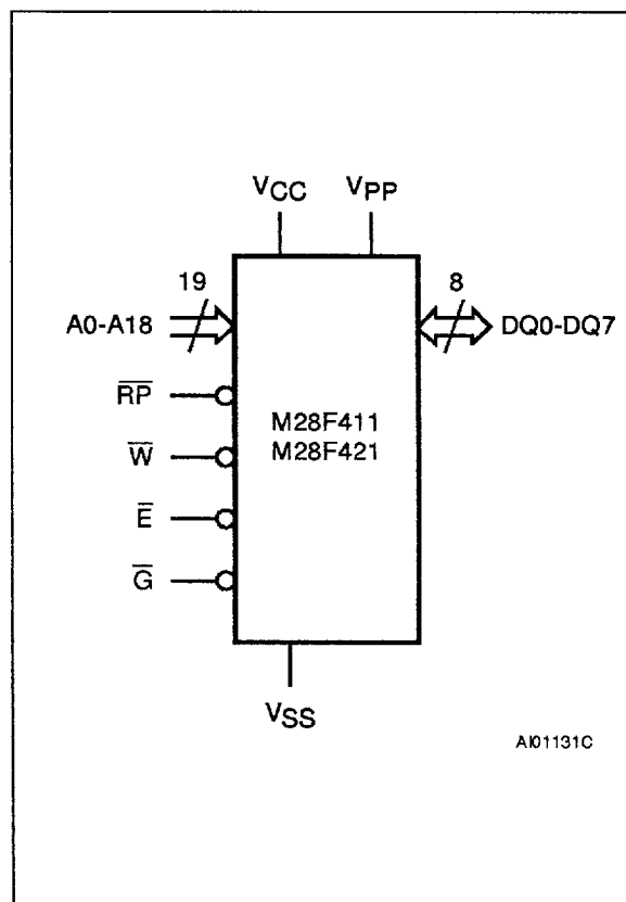
Figure 1. Logic Diagram
