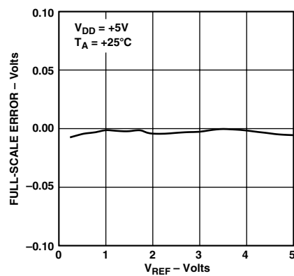
Figure 26. Full-Scale Error vs. V_{REF} (Buffered)
