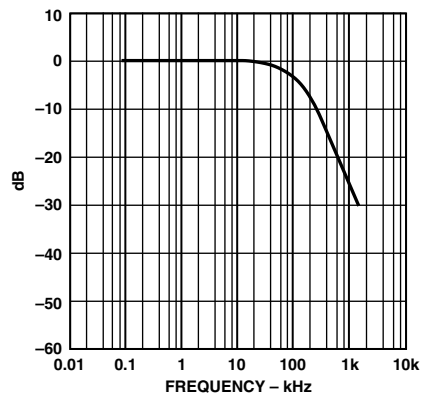
Figure 24. Multiplying Bandwidth (Small-Signal Frequency Response)
