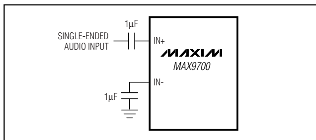
Figure 6. Single-Ended Input
