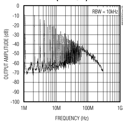
WIDEBAND OUTPUT SPECTRUM (FFM MODE)
