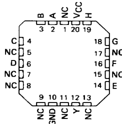
SN54LS55 ... FK PACKAGE SN74LS55 ... FN PACKAGE (TOP VIEW)
