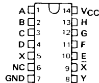
SN54H55 ... W PACKAGE (TOP VIEW)
