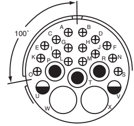
100° Rotation of 32-6 32-16 Service Rating A Number of Contacts 2 3 2 16 Contact Size 4 8 12 16
