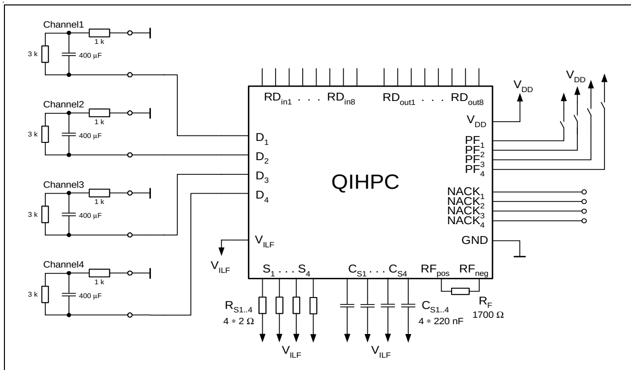
Figure 8 Circuit with “LT Power Source Test Loads”
