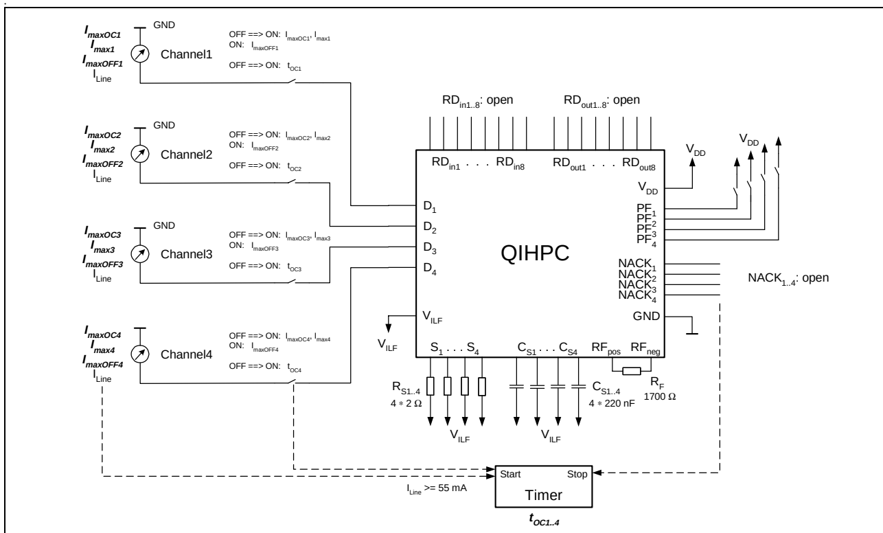
Figure 11 Line Currents and Delay Time t_{OC}
