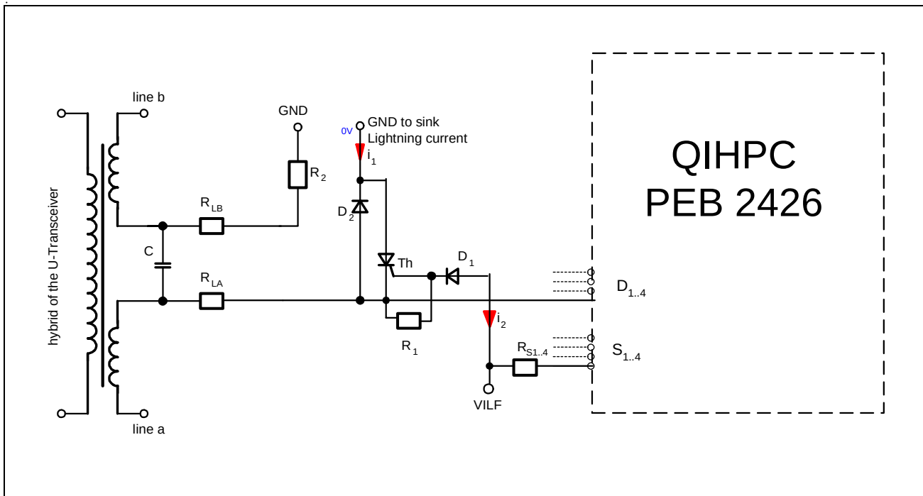
Figure 7 Proposal for a Protection Circuitry
