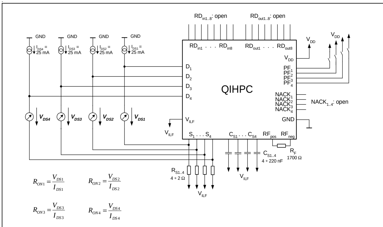
Figure 12 DMOS- R_{ON} resistance
