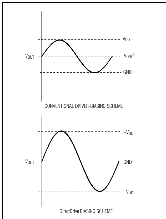
Figure 1. Traditional Driver Output Waveform vs. MAX4409 Output Waveform
