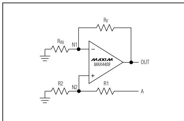
Figure 5. Common-Mode Sense Equivalent Circuit
