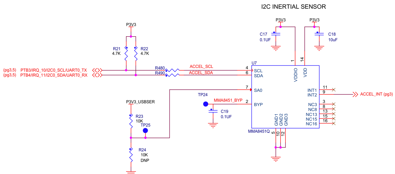
Figure 6. Accelerometer connection
