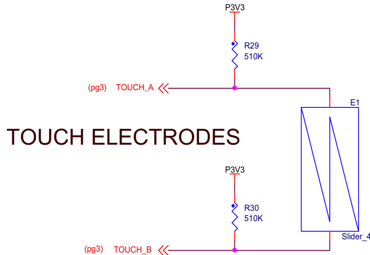
Figure 5. Touch slider connection
