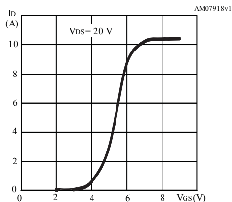
Figure 6. Transfer characteristics
