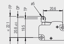
L11: Rollenhebel
