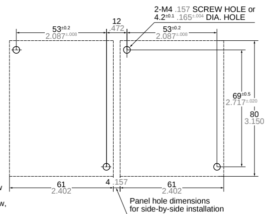
Mounting dimensions
