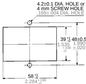
Rear surface-mounting
