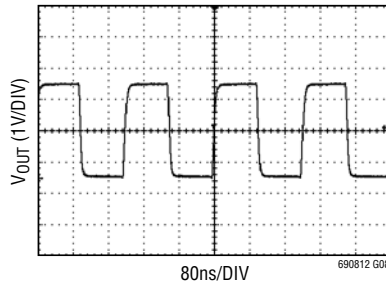
Output Operating at 5MHz, V^+ = 3\text{V}
