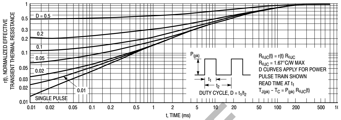
Figure 10. Thermal Response
