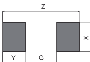
Dimensions [mm]
