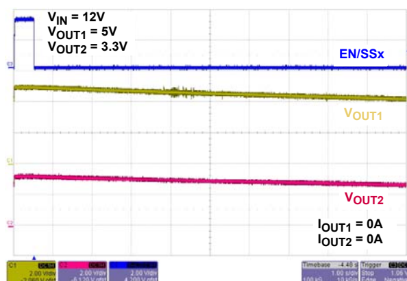
FIGURE 12. EN/SS SHUTDOWN
