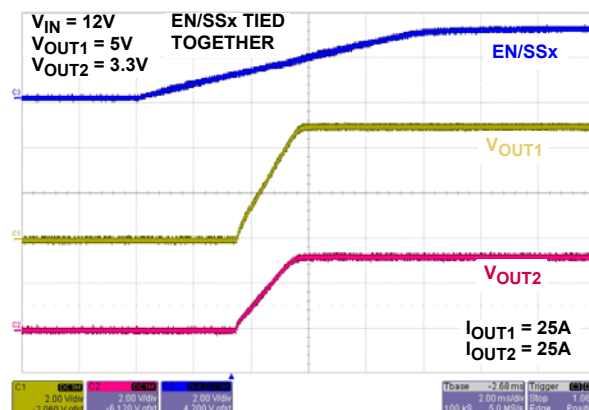
FIGURE 11. EN/SS START-UP
