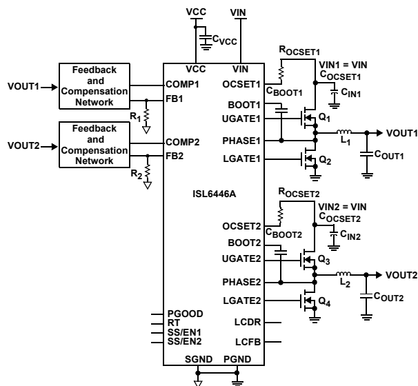
FIGURE 1. TYPICAL APPLICATION
