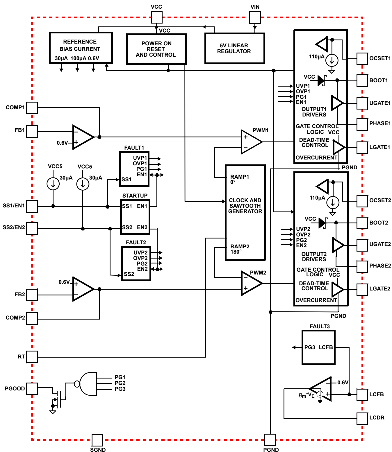
FIGURE 3. BLOCK DIAGRAM
