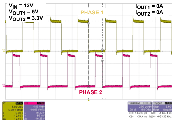
FIGURE 8. PWM INTERLEAVING
