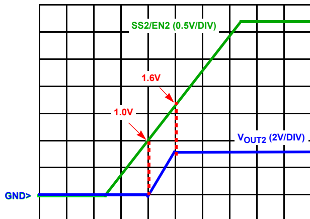
FIGURE 18. SOFT-START
