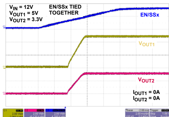
FIGURE 10. EN/SS START-UP
