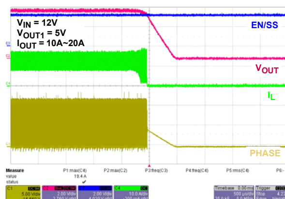
FIGURE 15. OVERCURRENT PROTECTION
