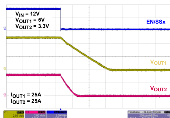
FIGURE 13. EN/SS SHUTDOWN
