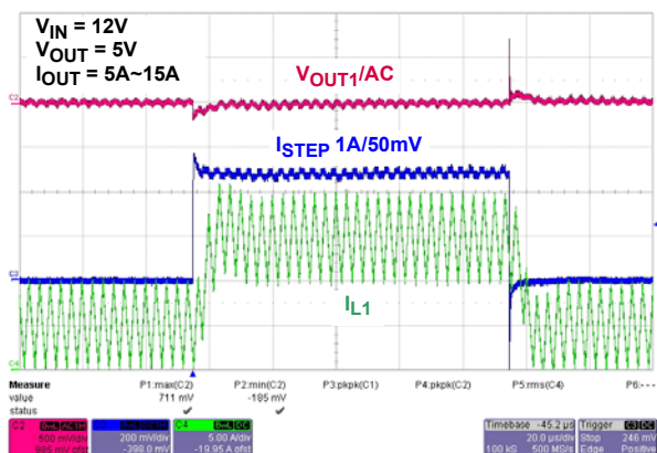
FIGURE 7. LOAD TRANSIENT
