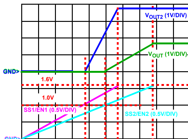
FIGURE 19. VOLTAGE TRACKING
