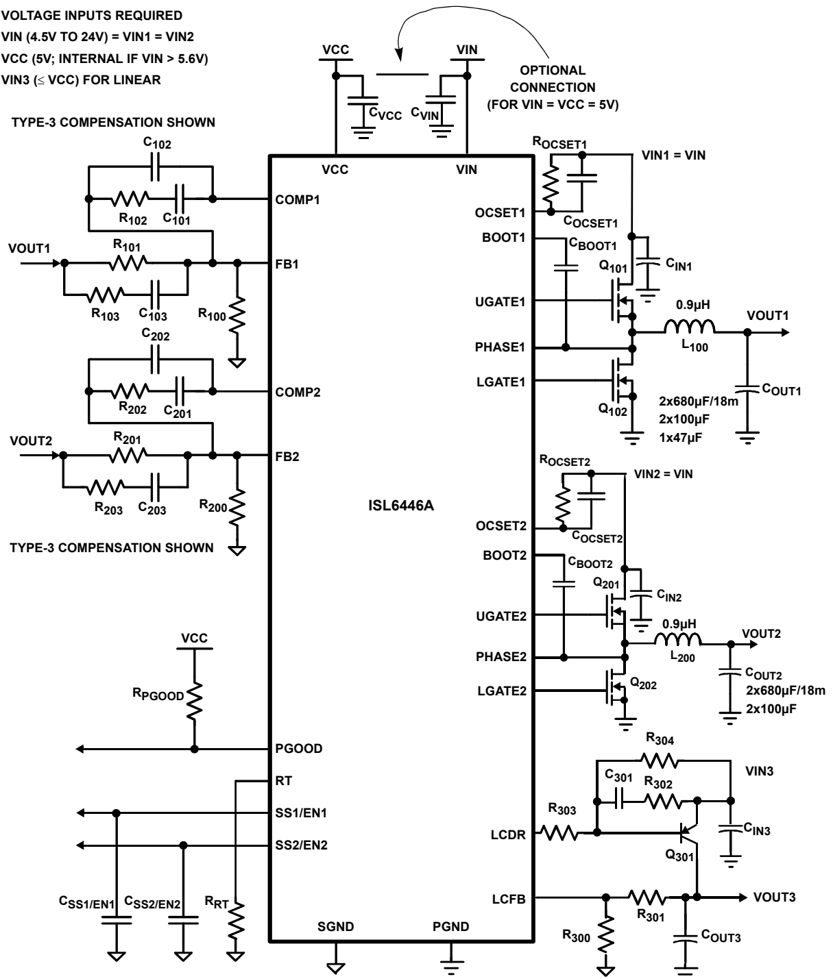
FIGURE 4. ISL6446A TYPICAL APPLICATION
