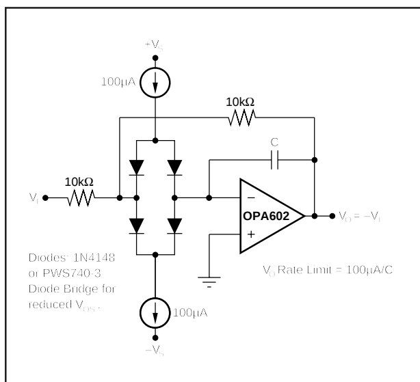
FIGURE 17. Rate Limiter.
