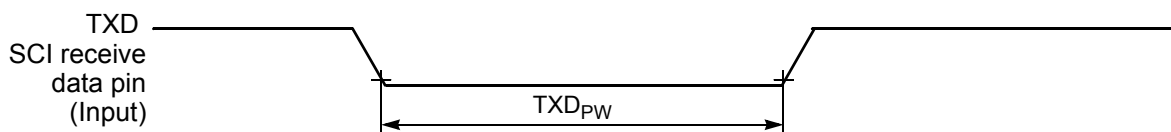
Figure 4-29 TXD Pulse Width
