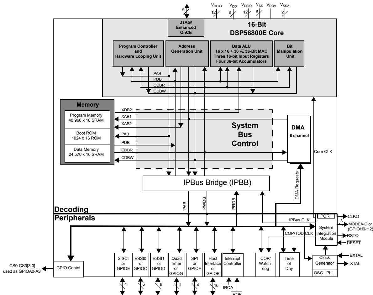
56857 Block Diagram
