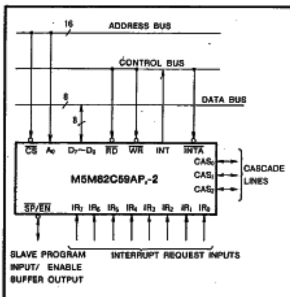
Fig. 1 The M5M82C59AP,-2 interfaces to standard system bus.
