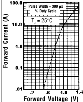
Typical Instantaneous Forward Characteristics
