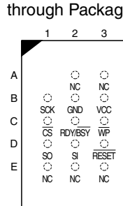
CBGA Top View through Package
