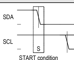
I 2 C Transmission Start Condition
