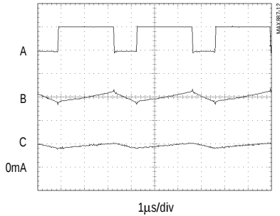
HEAVY-LOAD, PWM-MODE SWITCHING WAVEFORMS
