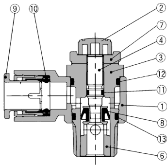
Meter-out
