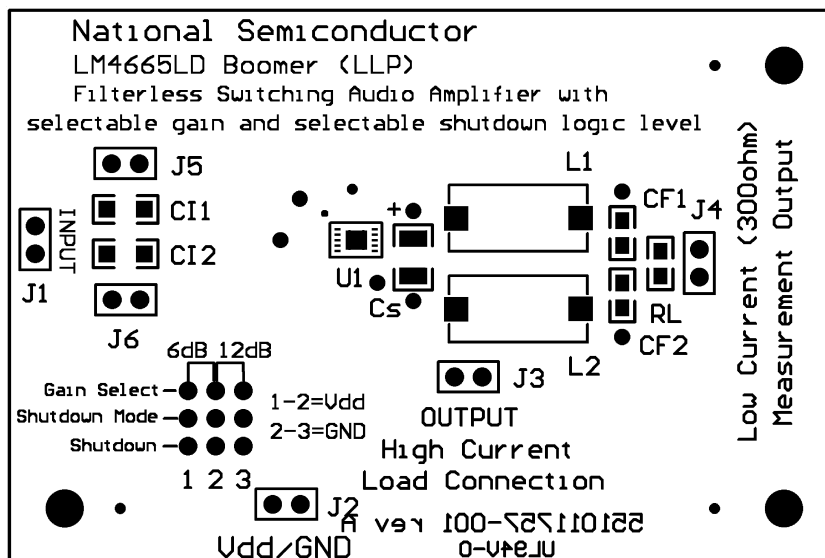
Figure 41. Silk Screen
