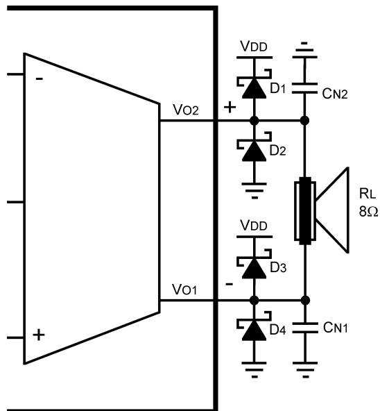
Figure 31. Increased Supply Voltage Operating Range for the DSBGA Package
