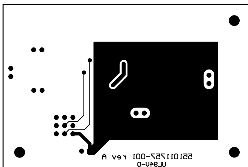
Figure 43. Bottom Layer
