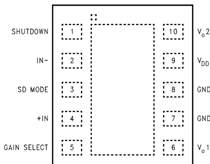
Figure 4. WSON Package – Top View See Package Number NGZ
