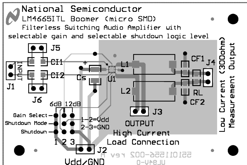
Figure 45. Silk Screen
