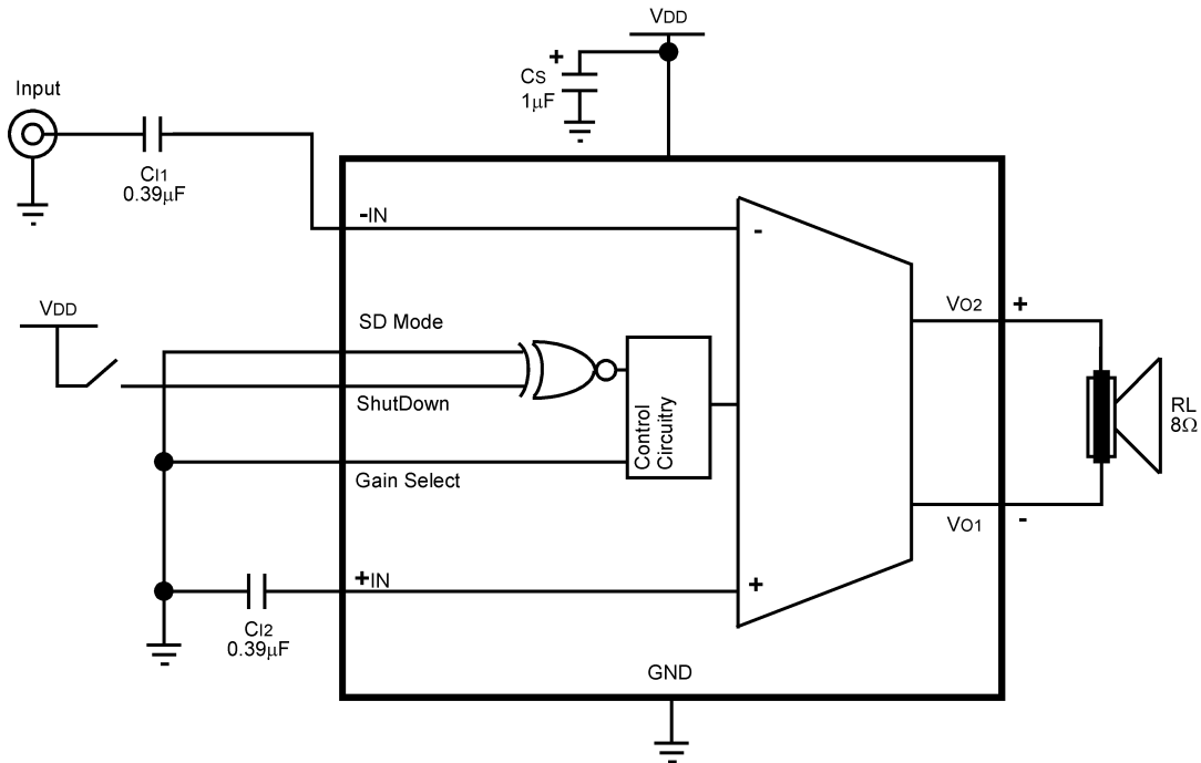
Figure 35. Single-Ended Input, Shutdown Low and Gain of 12dB Configuration
