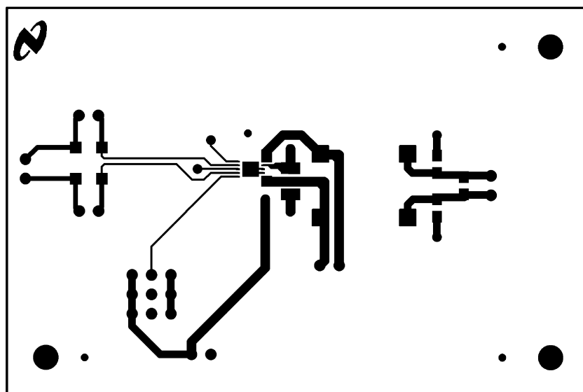
Figure 42. Top Layer
