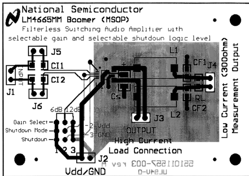
Figure 36. Composite View
