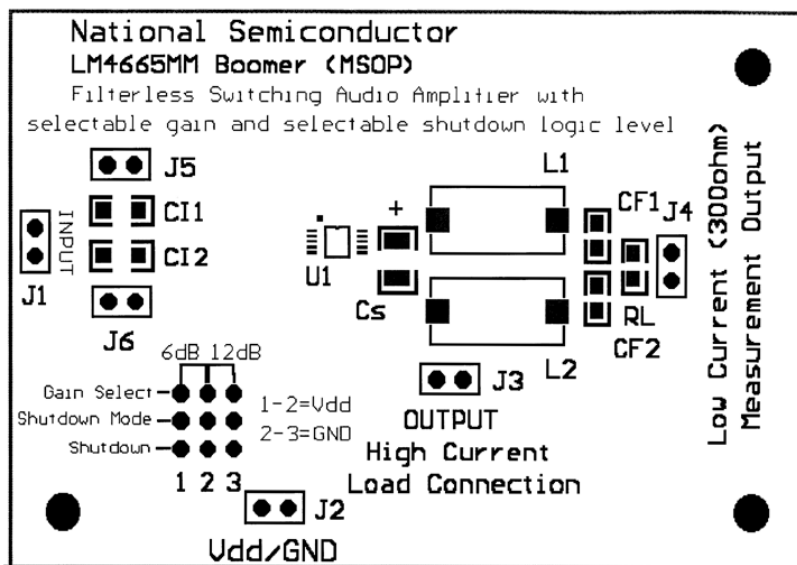
Figure 37. Silk Screen
