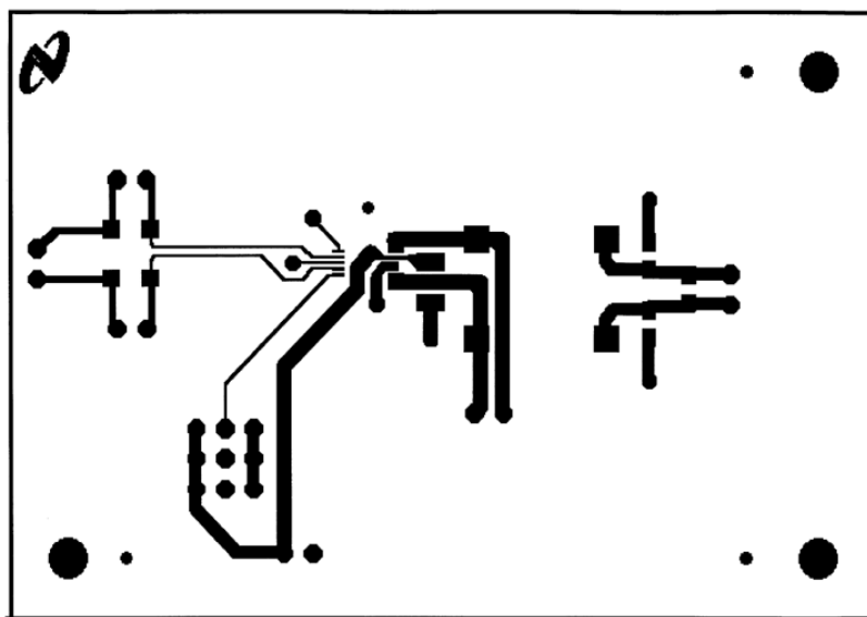
Figure 39. Bottom Layer
