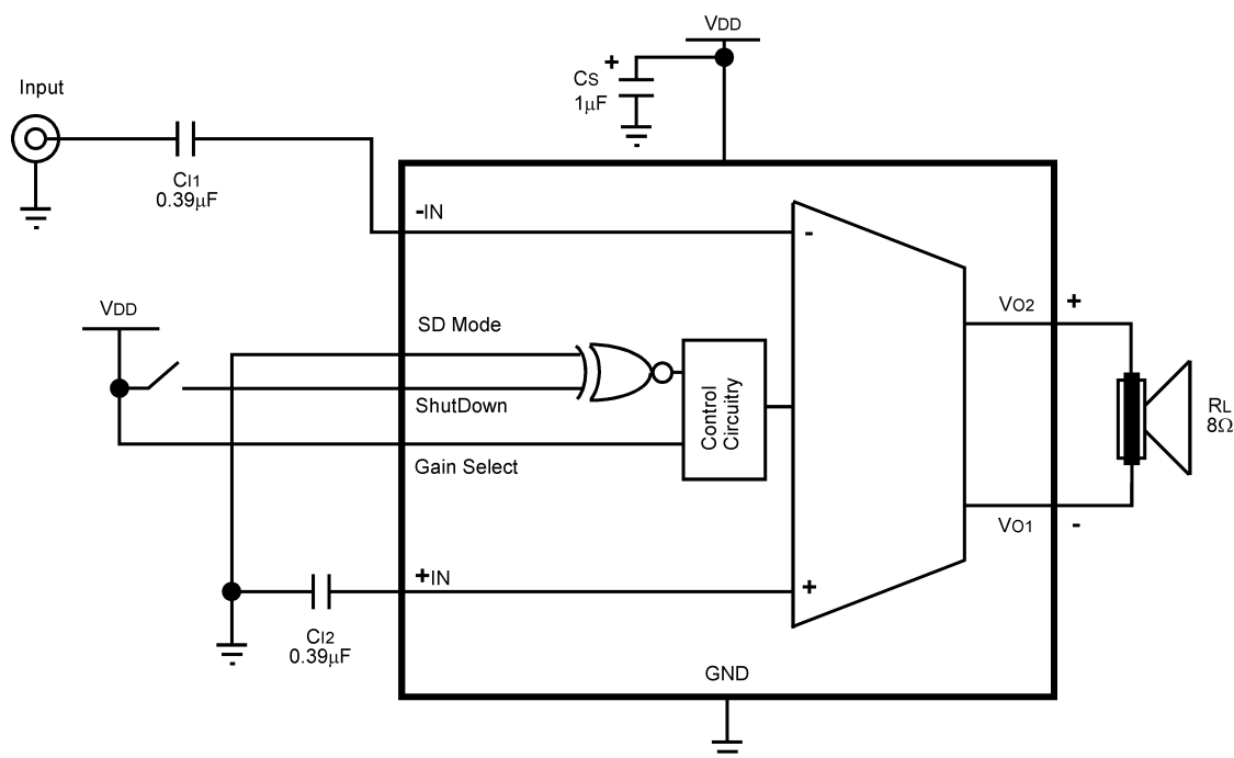
Figure 34. Single-Ended Input, Shutdown Low and Gain of 6dB Configuration
