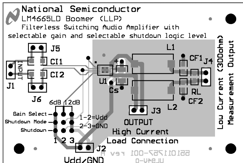
Figure 40. Composite View
