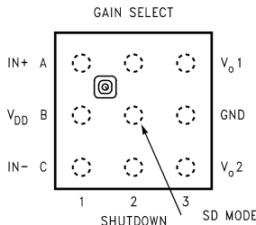
Figure 3. 9 Bump DSBGA Package – Top View See Package Number YZR0009
