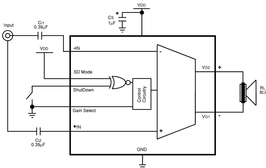
Figure 33. Single-Ended Input, Shutdown High and Gain of 12dB Configuration
