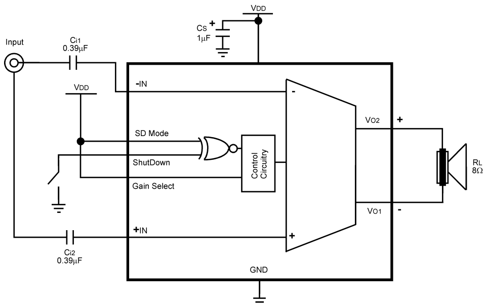
Figure 32. Single-Ended Input, Shutdown High and Gain of 6dB Configuration
