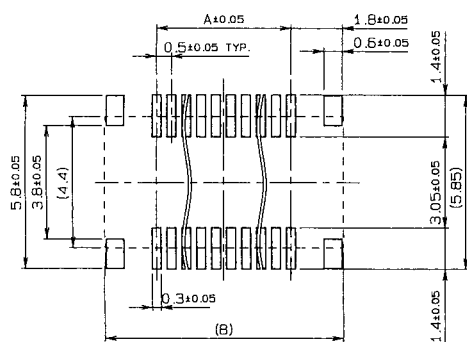
MOUNTING LAYOUT
