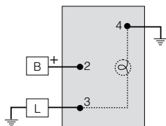
SPST Off-ON - Dependent Illumination (Three terminals) Diagram F
