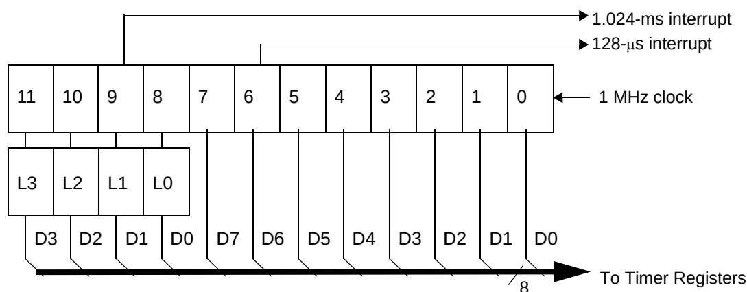
Figure 13. Timer Block Diagram
