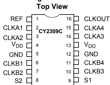
Figure 2. Pin Diagram - 16 Pin SOIC/TSSOP
