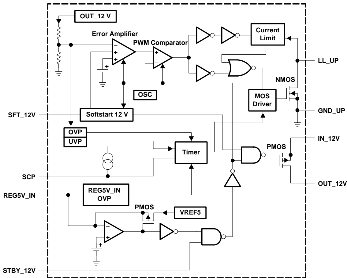
functional block diagram—boost 12-V block
