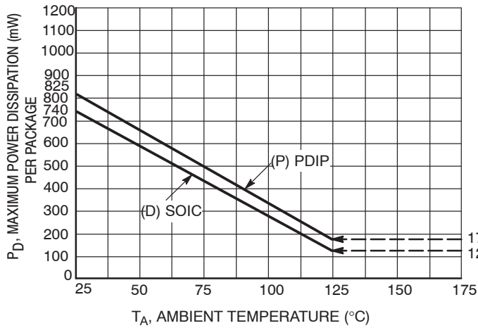
Figure 7. Ambient Temperature Power Derating
