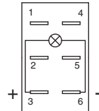
D - for function 1 (on-off) with LED on side A
