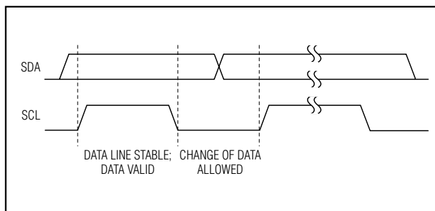
Figure 3. Bit Transfer
