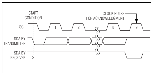
Figure 4. Acknowledge
