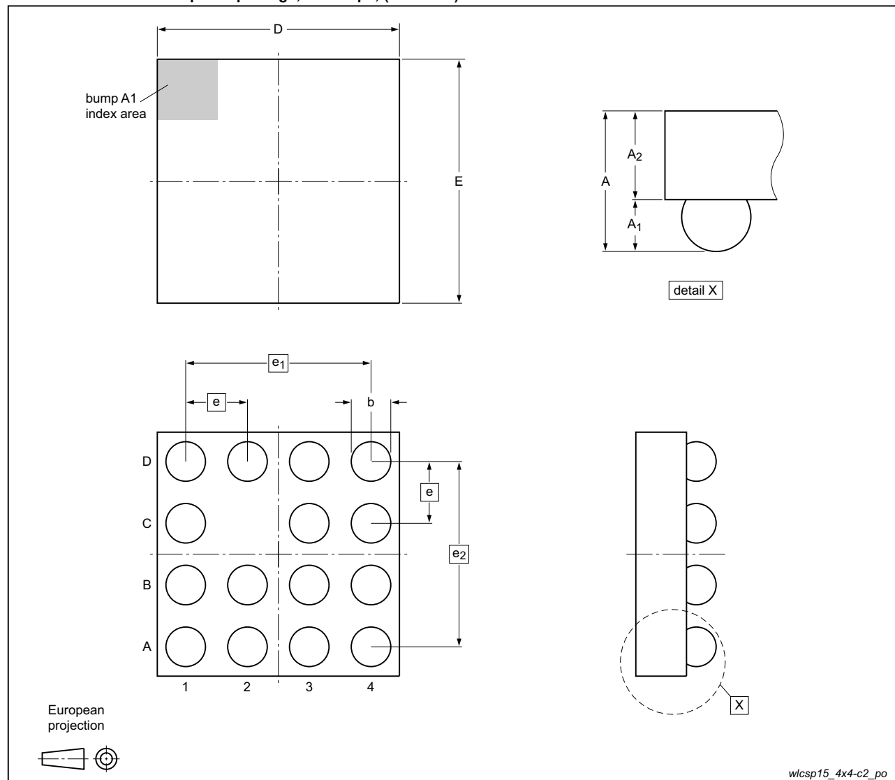
Fig 8. Package outline IP4340CX15 (WLCSP15)
