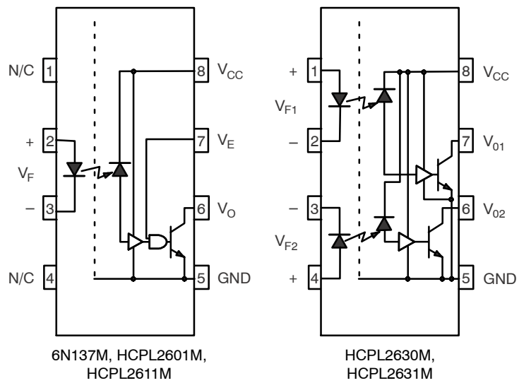
Figure 1. Schematics
