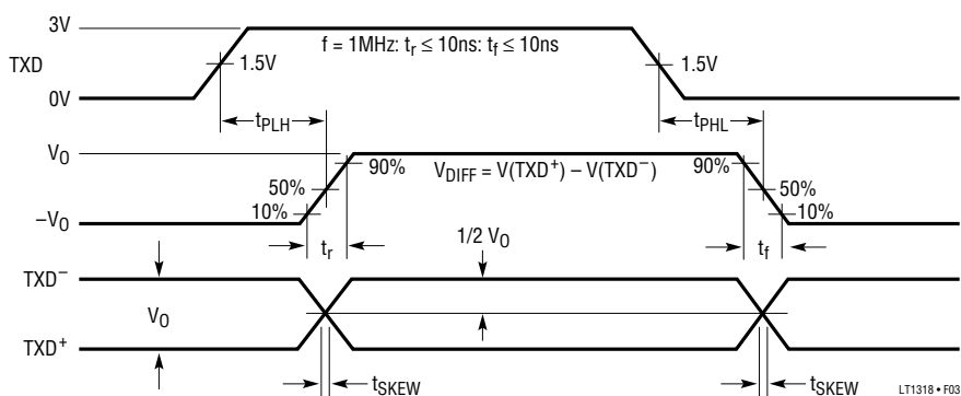
Figure 3. Differential Driver
